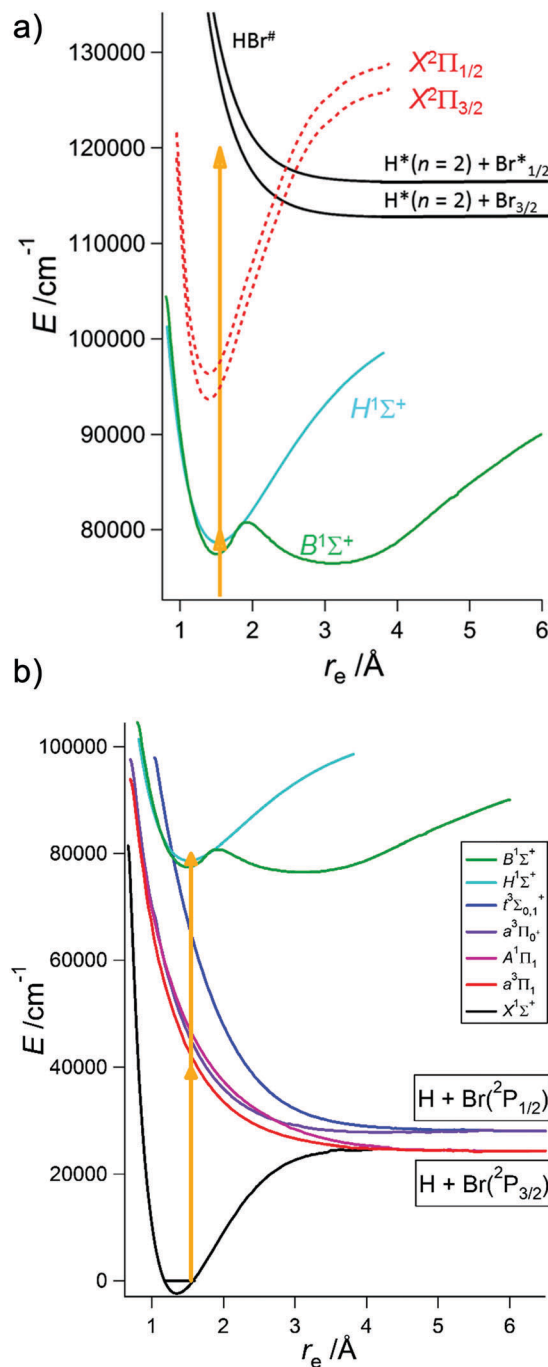
Fig. 9 (a) Potential curves of the states involved in the \text{H}^+ formation following two-photon resonance excitation of \text{HBr} to the \text{E}(v' = 1) , \text{H}(v' = 0) , \text{V}(v' = m + 8) and \text{V}(v' = m + 7) mixed states, asymptotic energies of fragments and relevant transitions (see main text). The potential curve for the B states (green solid curve) was derived from Fig. 1 in ref. 50. The potential curves for the ionic states (broken curves) were derived from ref. 56. The potential curve of the H state was derived from known origins of the v' = 0, 1, 2 states. 29 The shape of the repulsive states correlating with \text{H}^* + \text{Br}/\text{Br}^* and \text{H}^{**} + \text{Br} are based on preliminary ab initio calculations, 71 which suggest that the curves might be of shapes close to that of the \text{B}^2\Sigma ionic state. 71 (b) Potential curves of the states involved in the two-photon resonance excitation, asymptotic energies of the fragments detected by two-color experiments and relevant transitions (see main text). The relevant potential energy curves were derived from ref. 53.
