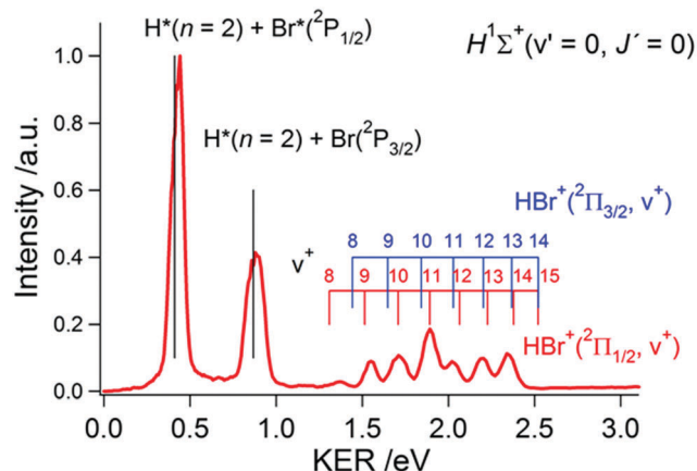
Fig. 5 \text{H}^+ kinetic energy release (KER) spectrum for resonance excitation from the ground state, \text{X}(v'' = 0, J'' = 0) to the \text{H}(v' = 0, J' = 0) state. Peaks corresponding to \text{H}^+ formation via the \text{Br}^* ( \sim 0.4 eV) and \text{Br} ( \sim 0.8 eV) channels (see main text) are marked. Predicted peak positions (assignments of peaks), with respect to the intermediate vibrational levels of the \text{HBr}^+/\text{HBr}^{*+} ionic states ( v^+ ) (1.3–2.5 eV) for the \text{HBr}^+ channels are also shown.
