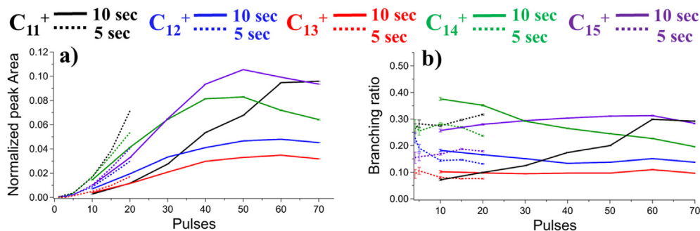
Fig. 9. Normalized mass peak areas (left panel) and branching ratios (right panel) corresponding to the C_{11}^+ – C_{15}^+ carbon clusters formed in the fragmentation of DBP for the 5 s and 10 s cycle pulse trains.
